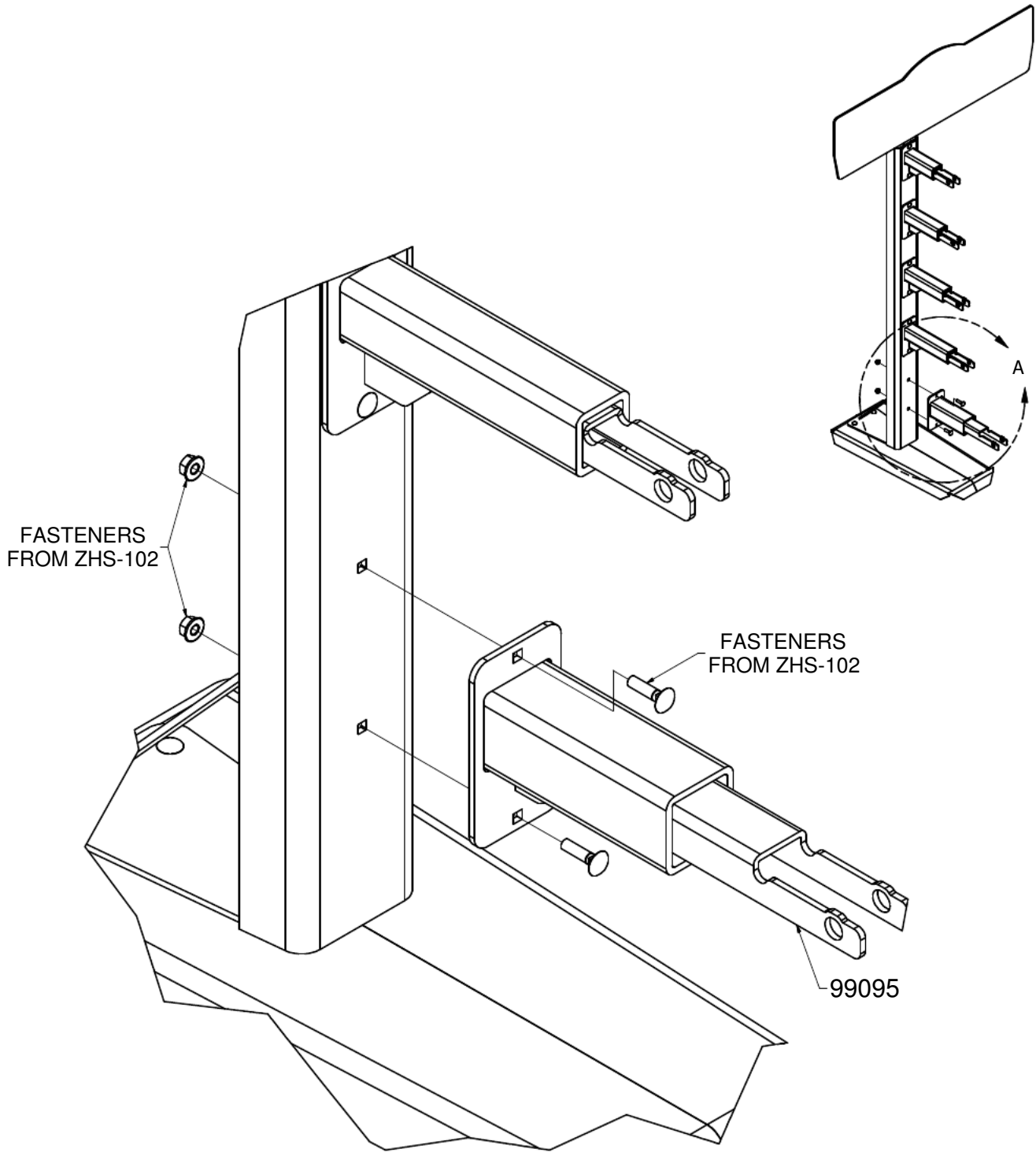
DETAIL A
