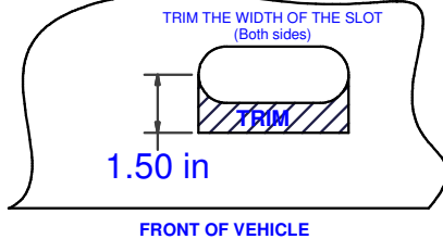
FASCIA TRIMMING DIAGRAM A (2011 and older models)
