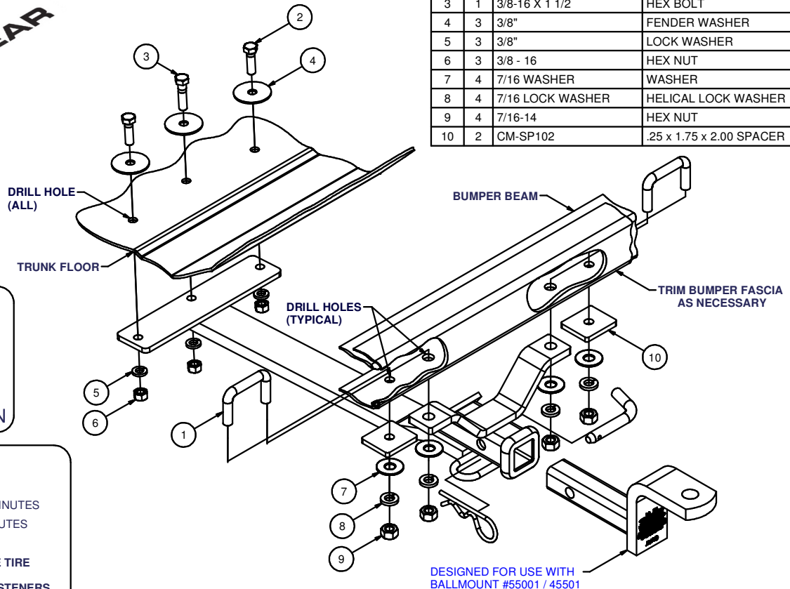
U-BOLT INSTALLATION
