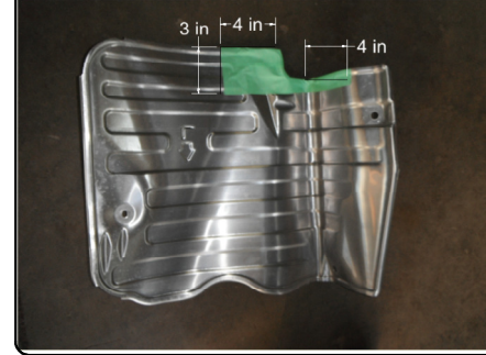
HEAT SHIELD TRIMMING DIAGRAM NOTE: TRIM DIMENSIONS ARE APPROXIMATE, CONFIRM FIT PRIOR TO TRIMMING.
