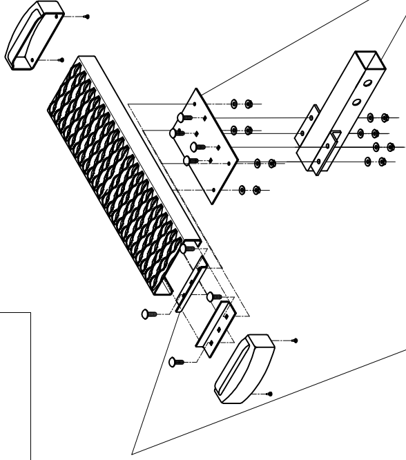
STINGER—PKG (570010)
