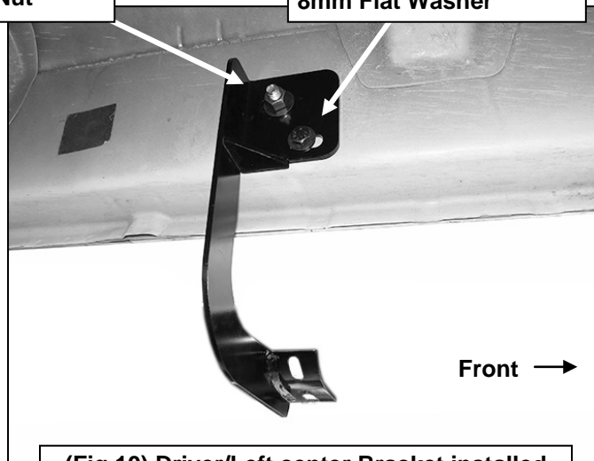
(Fig 10) Driver/Left center Bracket installed
